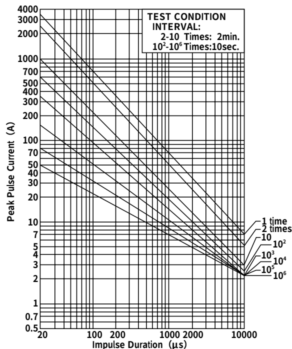
● TND10V-820K ~ TND10V-511K
